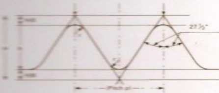
Fig. 1. (Parallel) H = 0.960491 \times p h = 0.640327 \times p r = 0.137329 \times p
