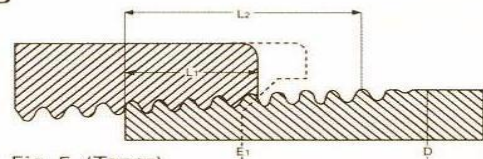
Fig. 5. (Taper) L_2 = (0.8D + 6.8) \frac{1}{n}
